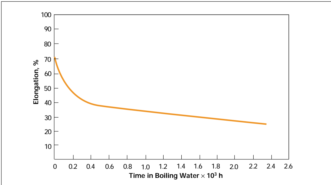
Figure 4. Ultimate Elongation After Exposure to 100°C (212°F) Water, Type HN Film, 25 µm (1 mil)
