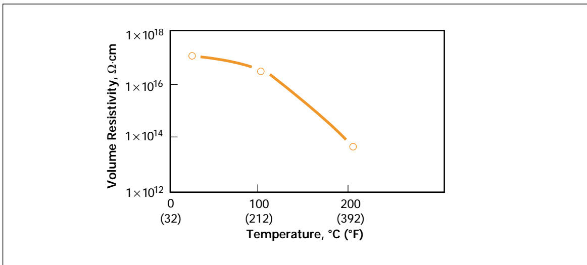
Figure 17. Volume Resistivity vs. Temperature, Type HN Film, 25 μm (1 mil)
