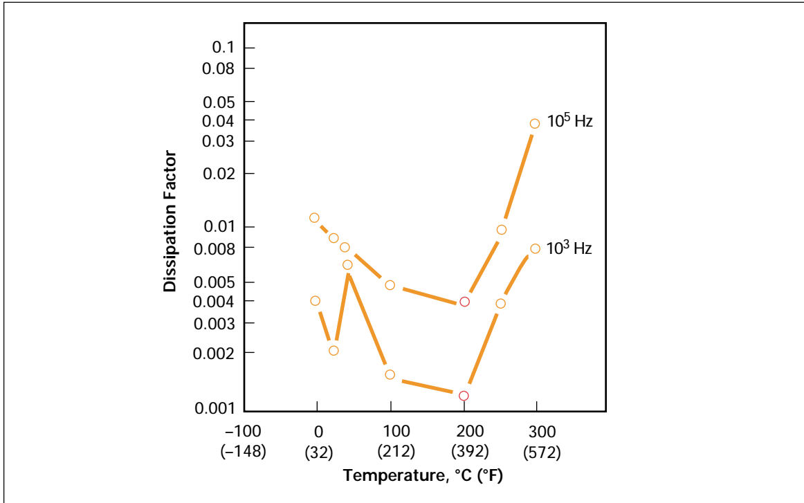
Figure 16. Dissipation Factor vs. Temperature, Type HN Film, 25 μm (1 mil)
