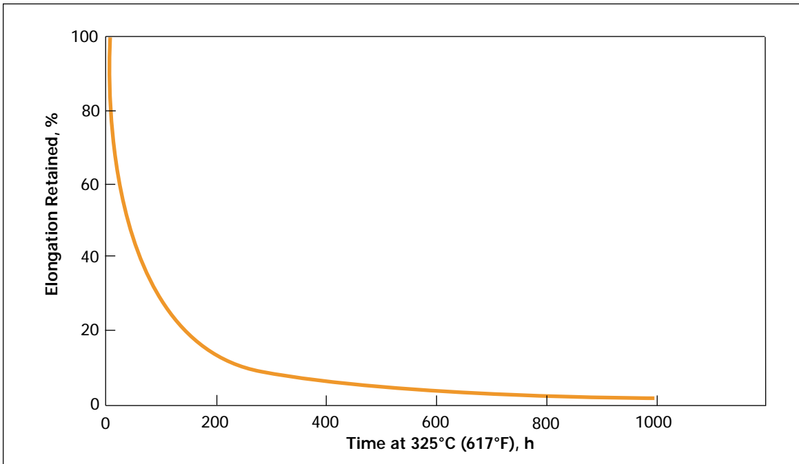
Figure 7. Ultimate Elongation vs. Aging in Air at 325°C (617°F), Type HN Film, 25 μm (1 mil)
